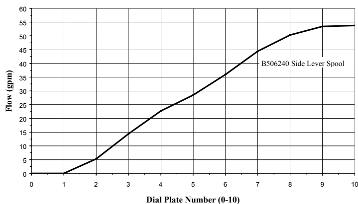
Flow vs. Dial Plate for FC51-1
