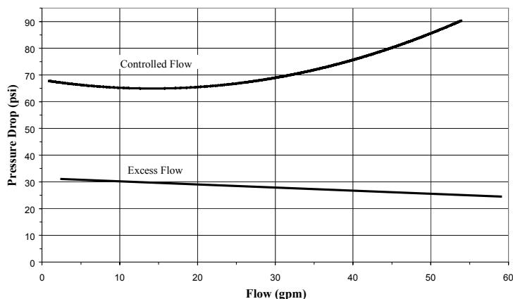
Pressure Drop vs. Flow for FC51-1
